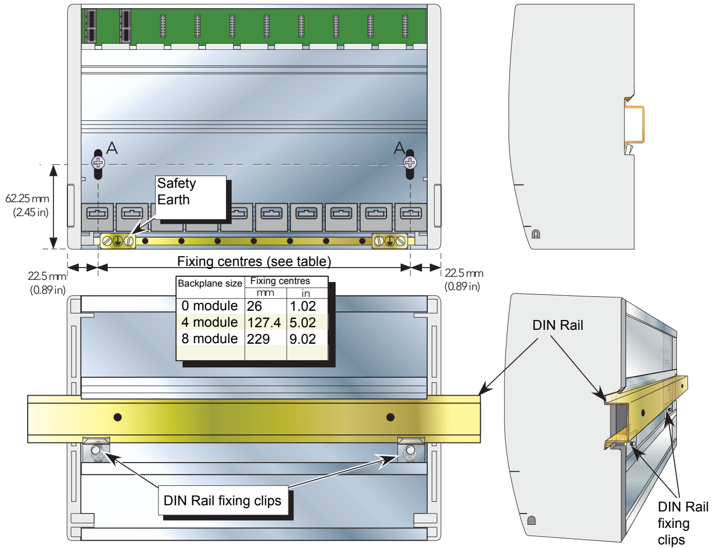
Figure 2: Fixing details (including safety earth connection)
