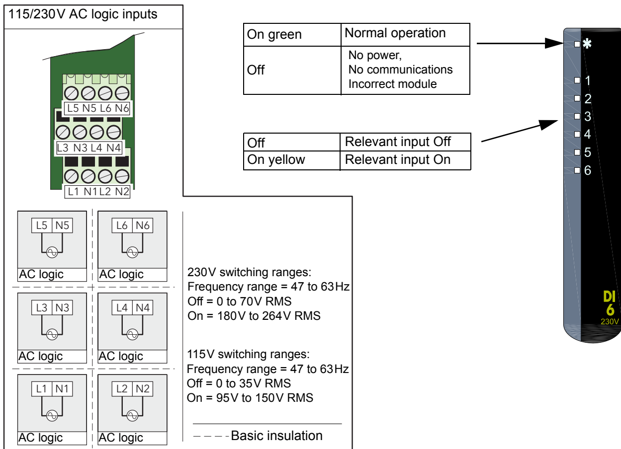
Figure 25: DI6 module pinout & status indicators (230V version shown; 115V version similar)
